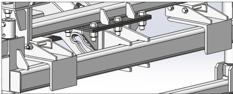
Figure 20: Adjusted Stopper Assembly
