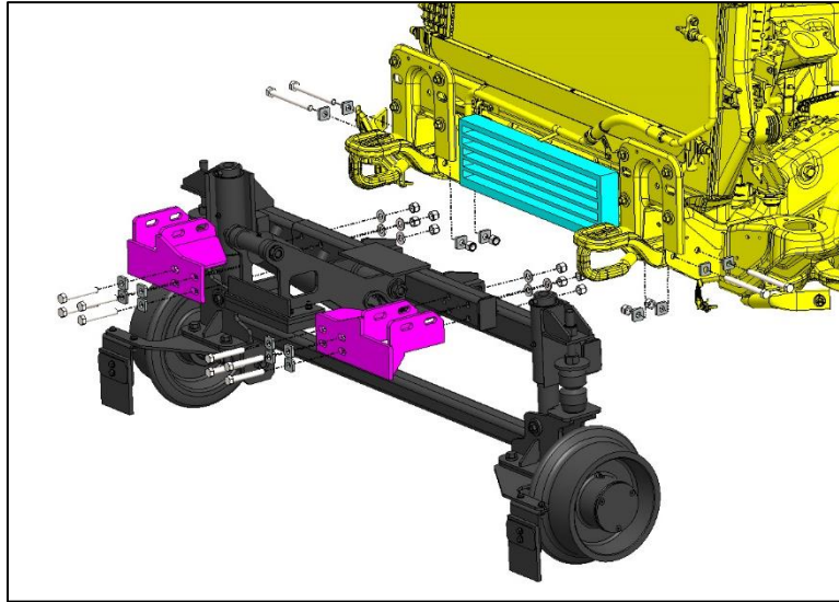
Figure 4: Front mounting plate removed
