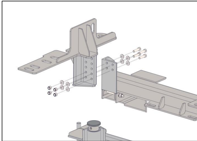
Figure 16: Height Adjustment Bolt Pattern
