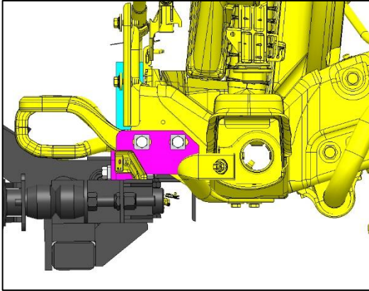
Figure 6: Front mounting plate positioned
