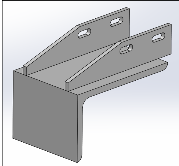
Figure 19: Stopper Assembly
