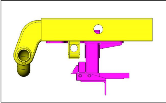
Figure 11: Rear mounting plate positioned
