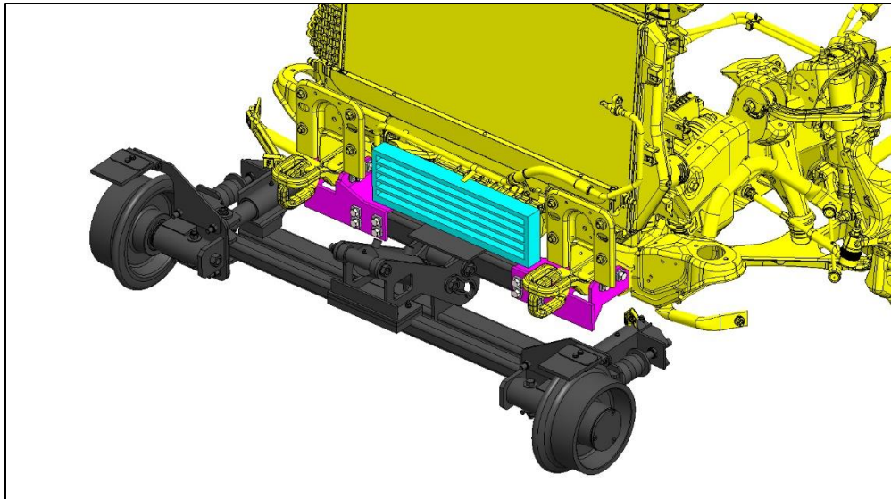
Figure 8: Front hi-rail installed
