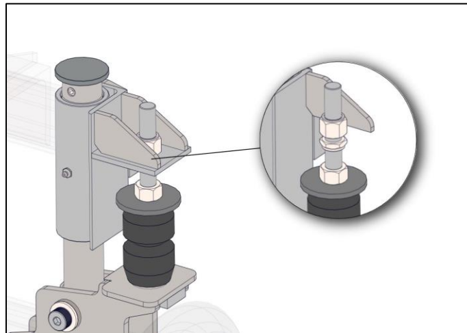
Figure 18: Wheel Weight Adjustment Threaded Rod
