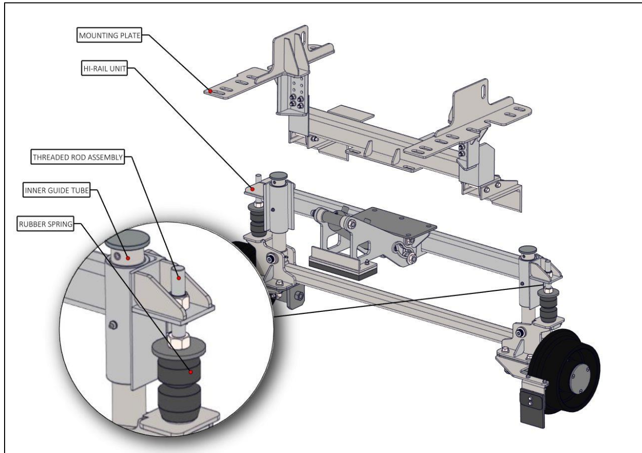
Figure 15: Rear Hi-Rail Assembly
