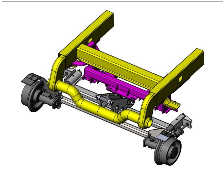
Figure 13: Rear hi-rail installed
